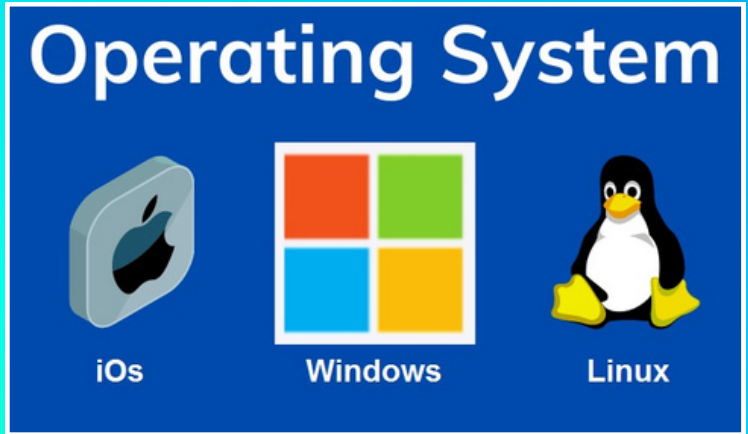
Operating System
